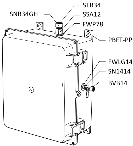
CONTROL BOX ASSEMBLY OUTSIDE VIEW
