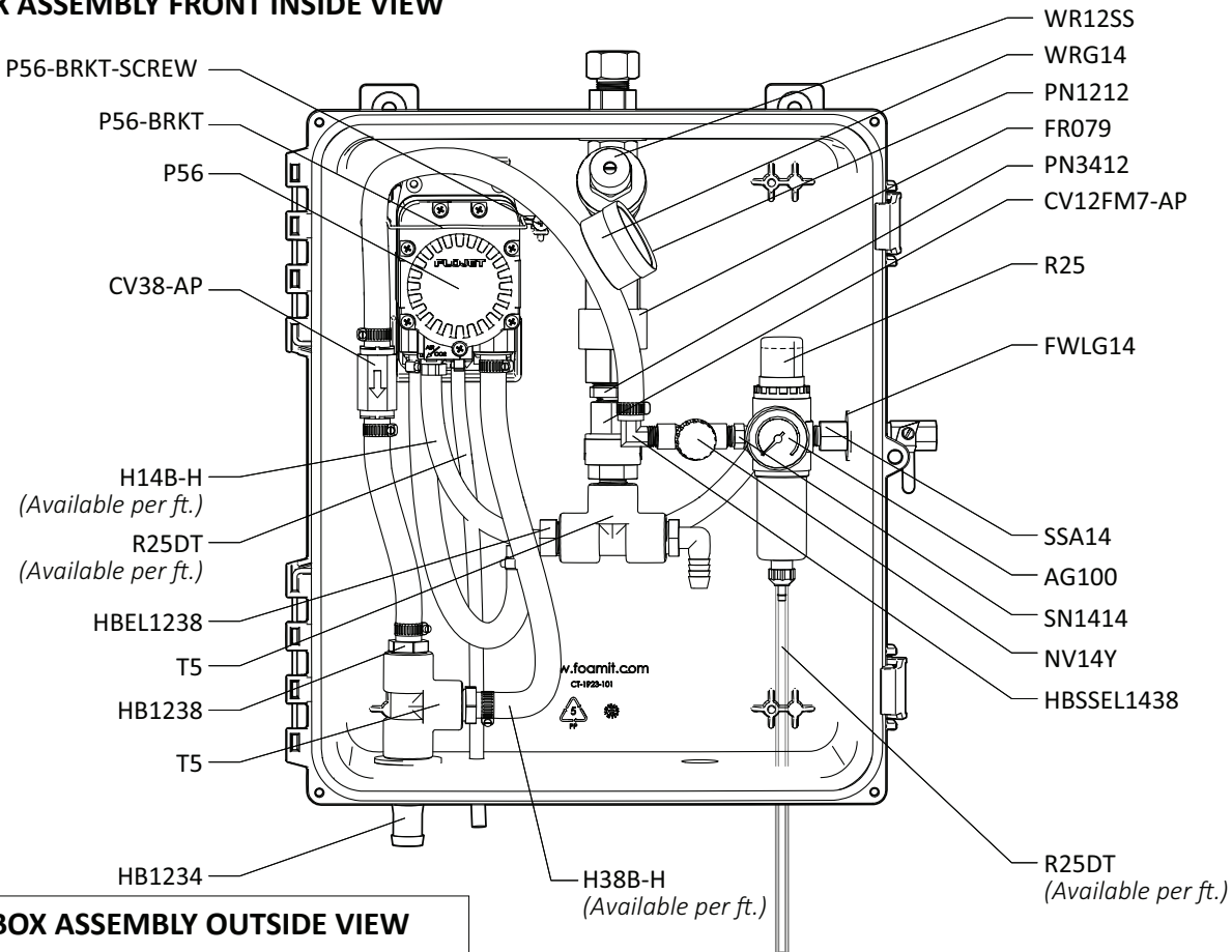
CONTROL BOX ASSEMBLY FRONT INSIDE VIEW
