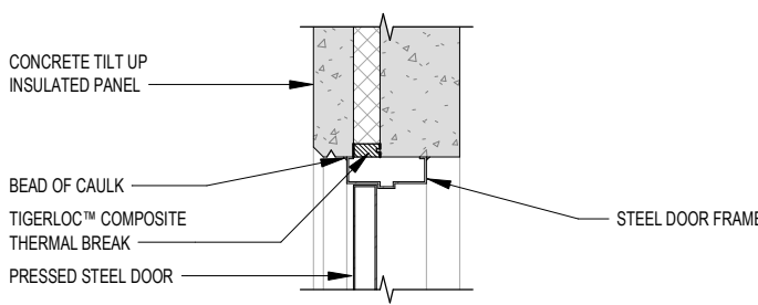
STEEL DOOR HEAD
