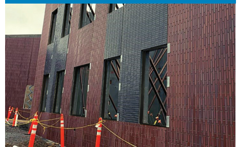
TIGERLOC PLUS SECURED INTO THE CONCRETE PANEL
