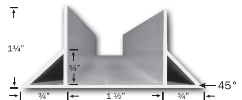
CLR HDCDL 3/4" High Double Chamfer
