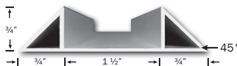
CLR DCDL 3/4" Double Chamfer
