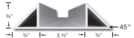
CLR DCEL 3/4" Double Chamfer
