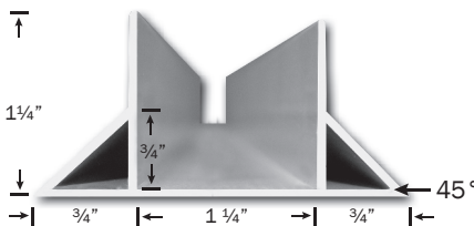
CLR HDCEL 3/4" High Double Chamfer
